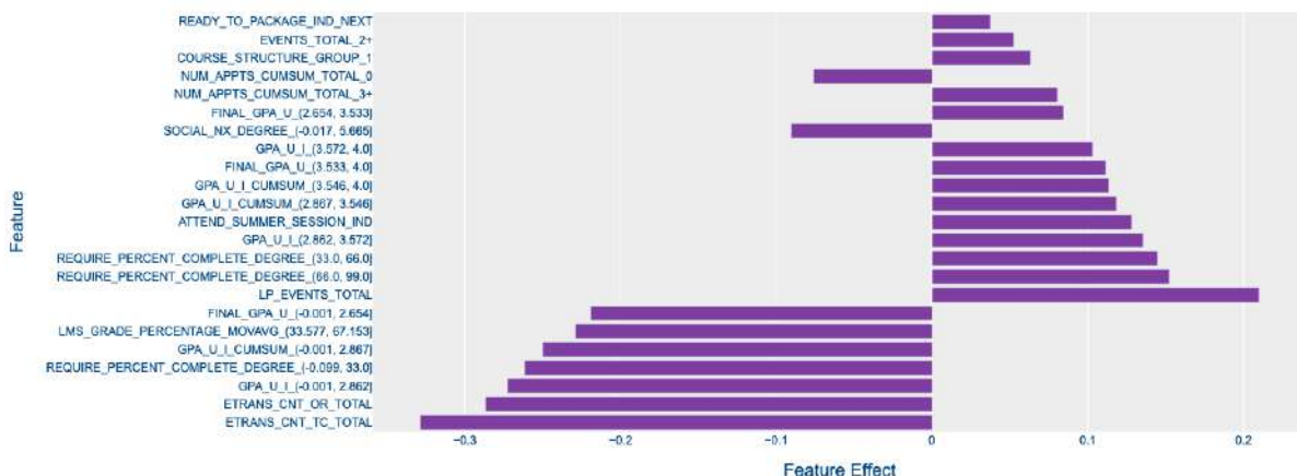
Figure 3. Feature Analysis
