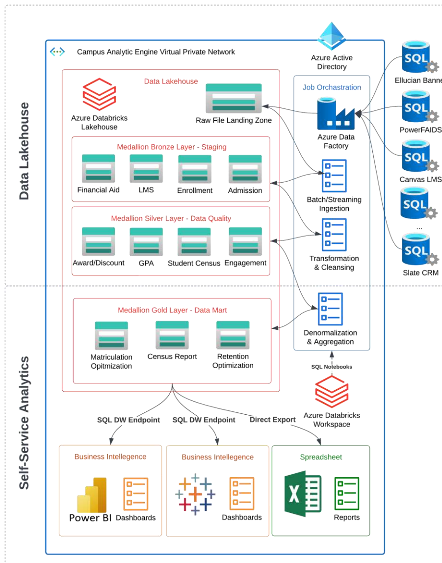
Figure 1. Example Architecture (Azure Cloud with Databricks Ecosystem)
